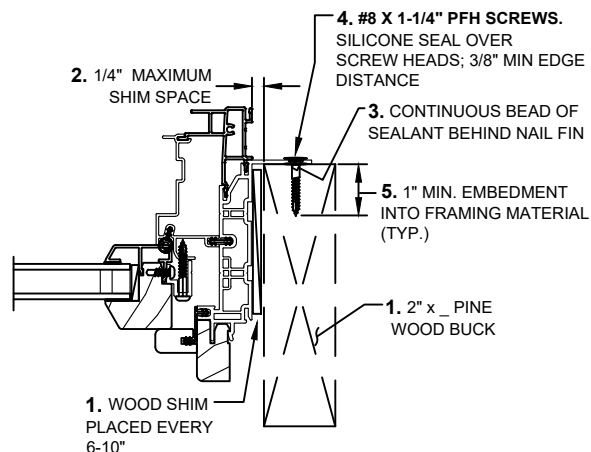
JAMB DETAIL H3 2.0 PICTURE / TRANSOM DOUBLE HUNG (4 9/16" JAMB)
