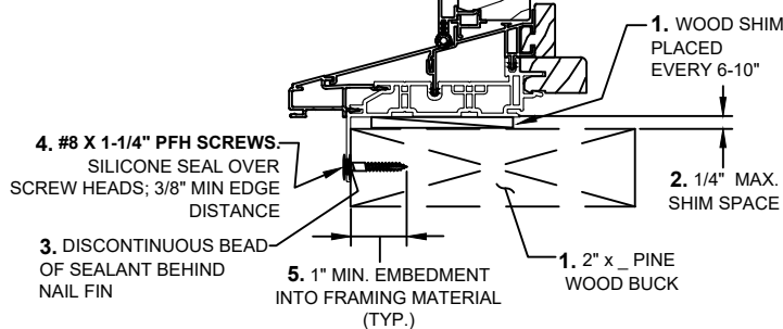
SILL DETAIL H3 2.0 PICTURE / TRANSOM DOUBLE HUNG (4 9/16" JAMB)
